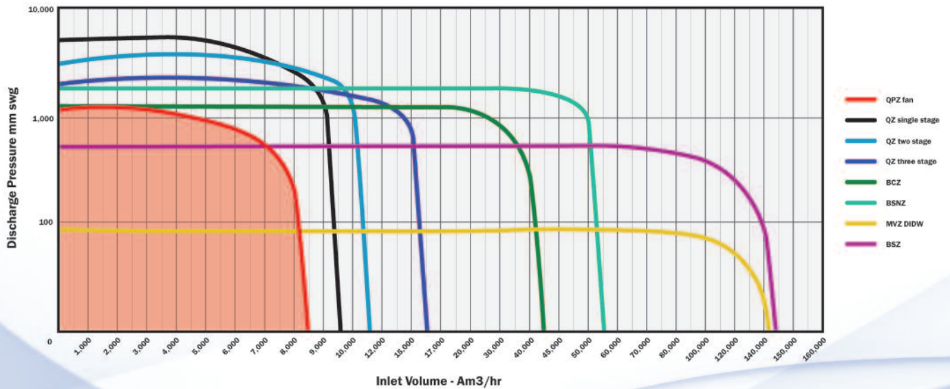
Fans & Blowers Range Performance Data
